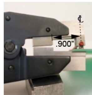
Figure 2: Wire Placement in Tool
