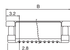
Without bosses
