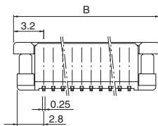
Without bosses
