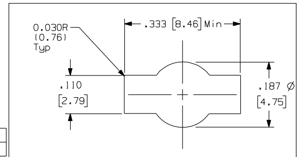
Typical PCB Mounting Configuration
